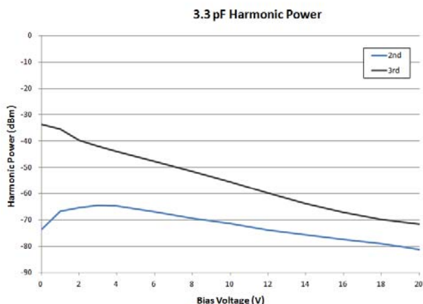
Figure 3. Harmonic Power
